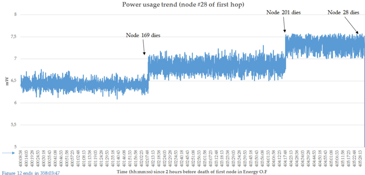
Fig. 13. Power consumption trend for the oldest node of first hop, detailed since 2 h before the first neighbour's battery exhaustion happens, in the case of Energy O.F. Experiment, which happens several hours later than previous figure.
