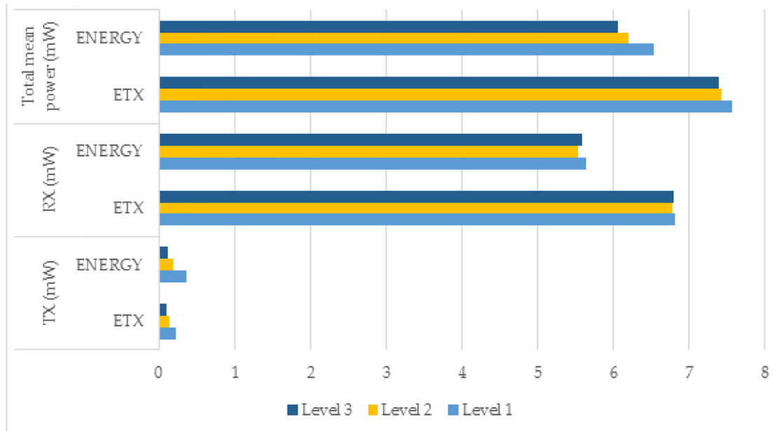
Fig. 11. Relevant power consumption profiles achieved during test.
