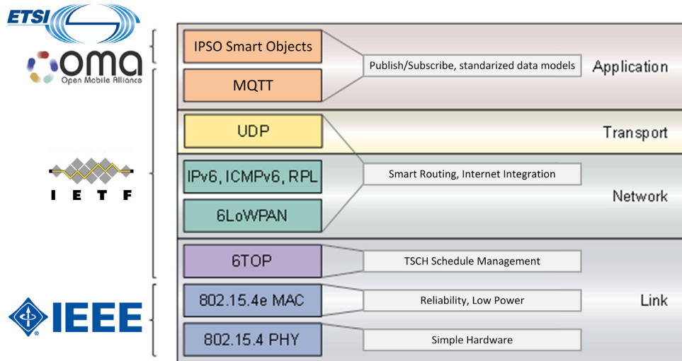
Fig. 6. Full protocol stack used for Deploy&amp;Forget WNS.
